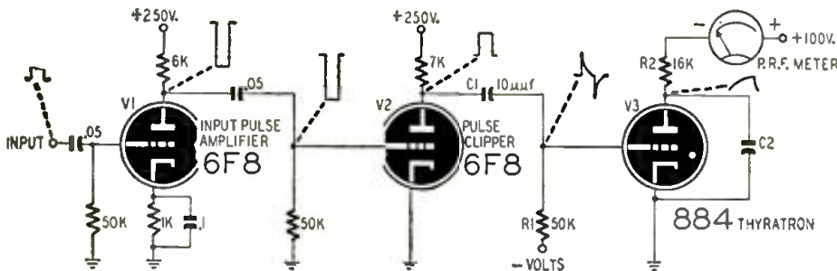
Fig. 3—Circuit of the pulse repetition frequency counter. Thyratron detail shown below.
