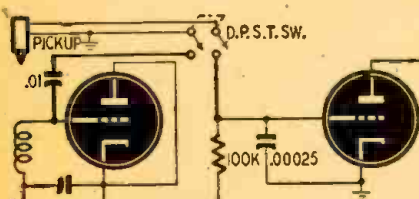
Fig. 3—Connection to sets like Philco III.
