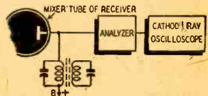
Fig. 4—Receiver mixer analysis connection.
