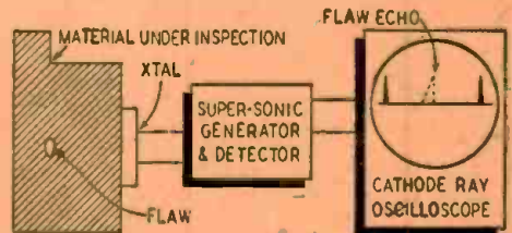
Fig. 4—Supersonic casting inspection hookup.
