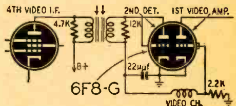
Fig. 3—Modification used in G.E. receivers.
