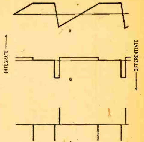
Fig. 4—A special-shaped wave differentiated.
