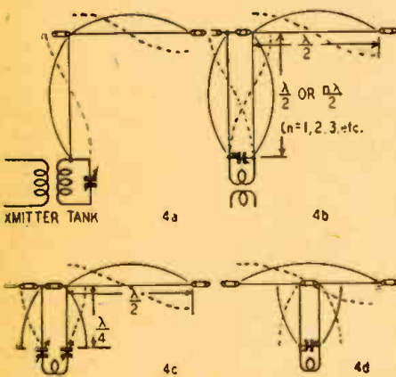
Fig. 4—Different types of transmission lines.
