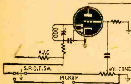
Fig. 1—Attachment to modern radio receiver.
