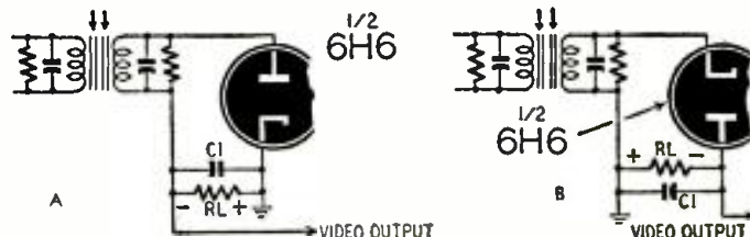
Fig. 6—Detector adjustments to insure positive picture polarity.
