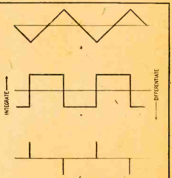
Fig. 2—Differentiation and integration in actual radio circuits.
