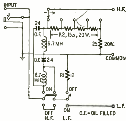
Fig. 5—A simple cross-over network.
