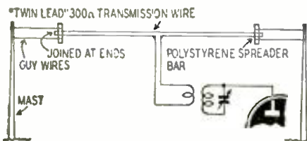
How the transmission-line antenna is erected.
