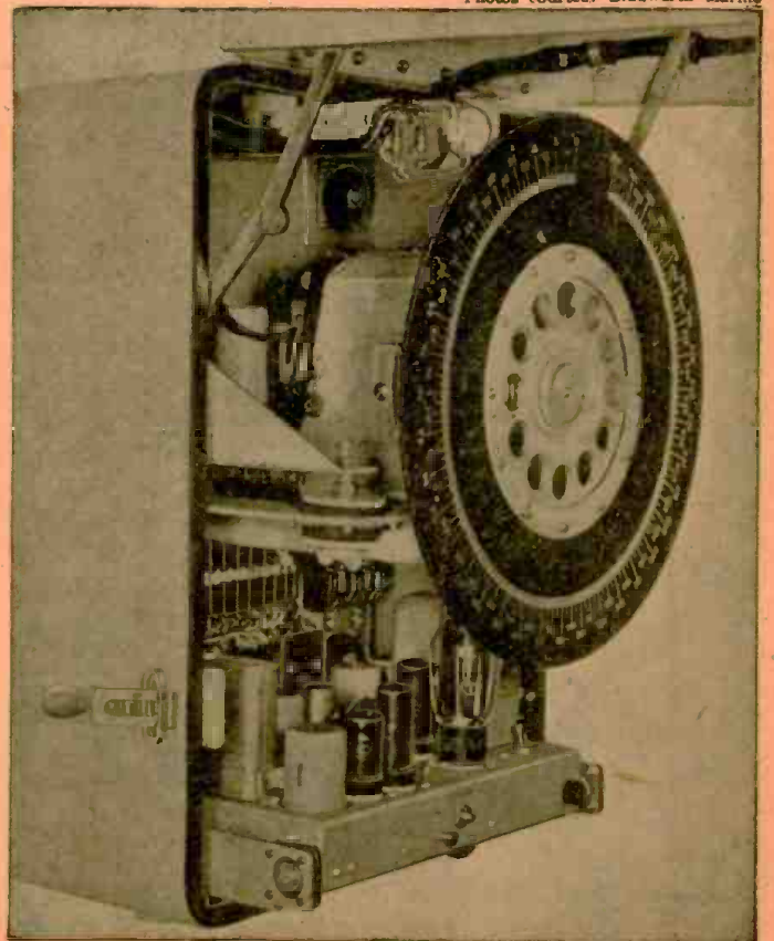
Photo D—This type of indicator has a fixed scale and moving light.
