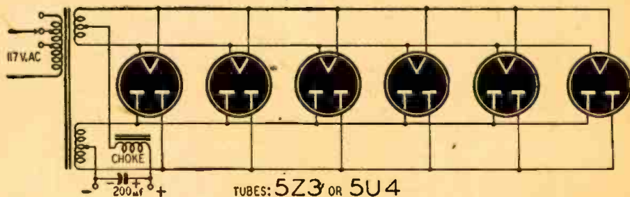
Fig. 2—A large bank of rectifiers excites the fields of several loudspeakers in parallel.
