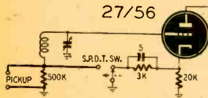
Fig. 2—Simple connection to power detector.
