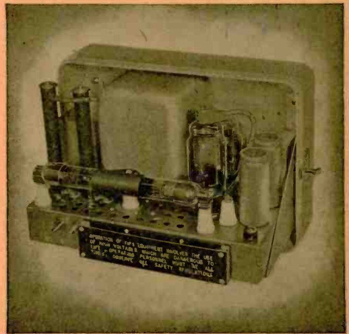
Photo B—A condenser-discharge type of supersonic signal generator.
