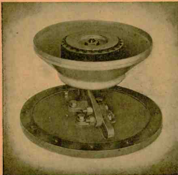
Photo A—Magnetostriction transducer used in underwater equipment.
