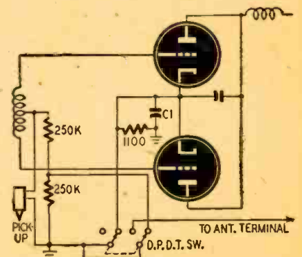
Fig. 5—Attachment to another special circuit.
