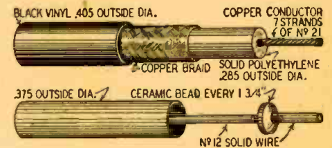
Fig. 6—Two types of popular co-axial cable.
