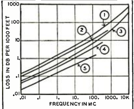
Fig. 7—Characteristics of co-axial cables.
