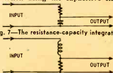
Fig. 8—This integrator employs an inductor.
